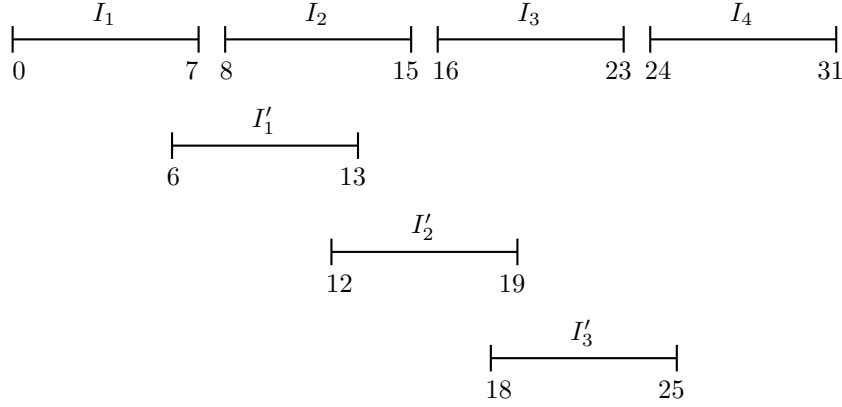
Figure 2: The intervals I_j, I'_j in the case r = 3 .
