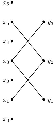
Figure 3: A Hasse diagram for the poset P with r = 6, s = 4, q = 6 . Figure 4 gives a unit point-core representation for P , showing it is a split semiorder.
